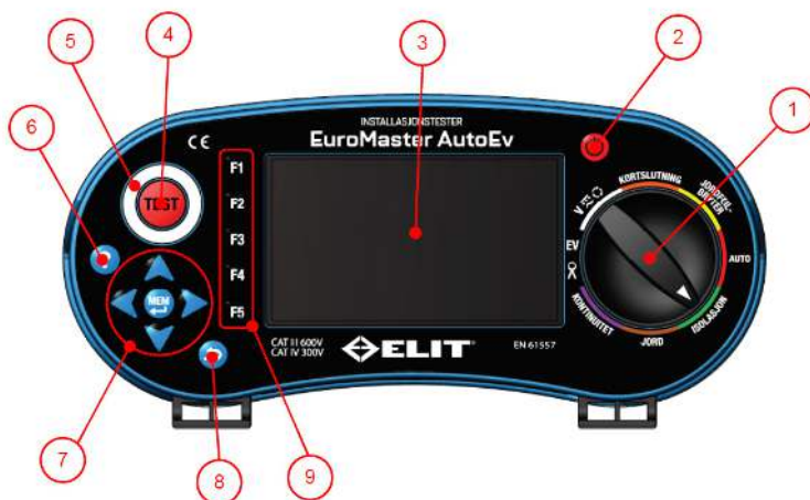
Figur 5.1 Front
