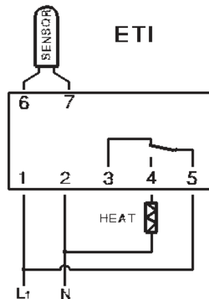
Wiring diagram
